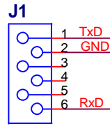
RJ11-6
